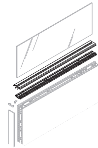
Frameless Glass Bottom Rail
