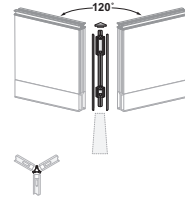
Full Panel — Trim and Corner Connectors — Steel, Aluminum, Wood
