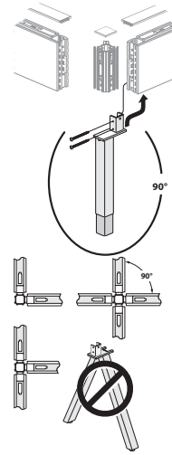
Beam Frame Leg — Straight Leg — 2-, 3-, 4-Way Intersection
