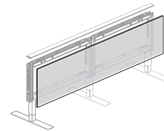
Tiles – Full Panel, Connections and Stack Frame
