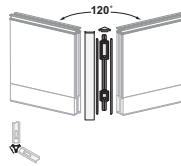
Full Panel — Trim and Corner Connectors — Work Rail
