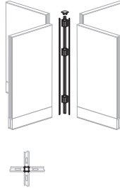
Full Panel — Trim and Corner Connectors — Steel, Aluminum, Wood
