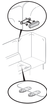
S9G-10 Ganging Kit
